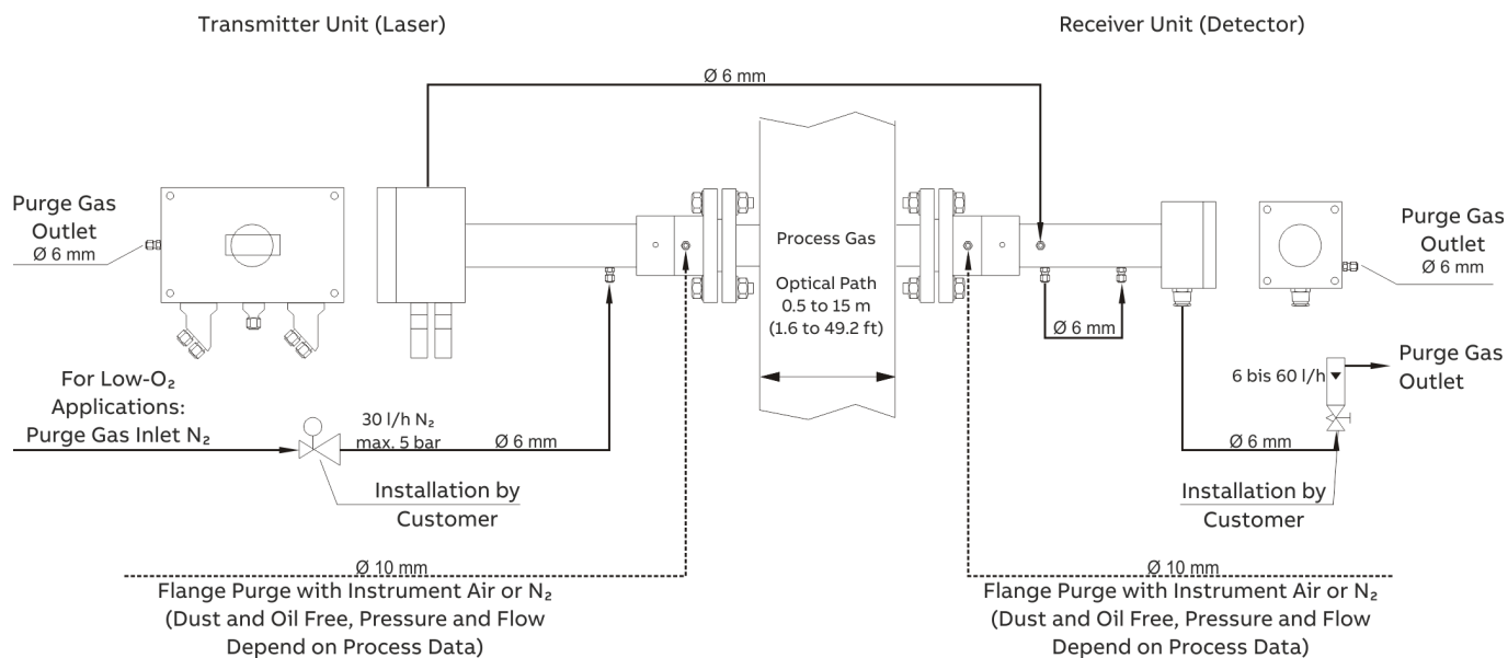
Figure 3: Purging of the transmitter and receiver units
