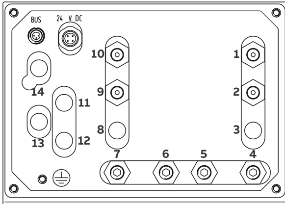
Figure 9: Gas connections Magnos27
