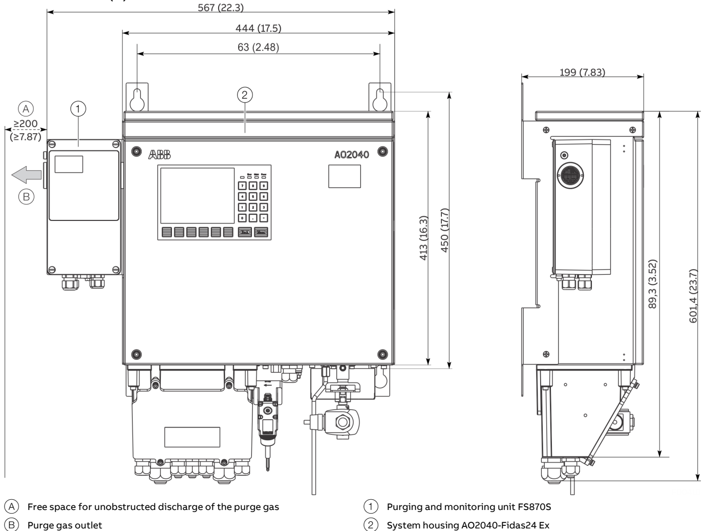
Figure 27: Dimensions, Model AO2040-Fidas24 Ex
