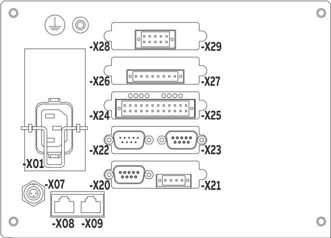
Image 18: Terminal assignment of electronic module (example)
