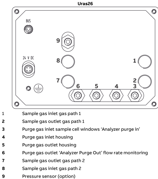
Figure 16: 'Safety Concept' gas connections Uras 26, Magnos28
