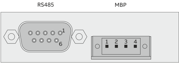
Image 19: PROFIBUS® module
