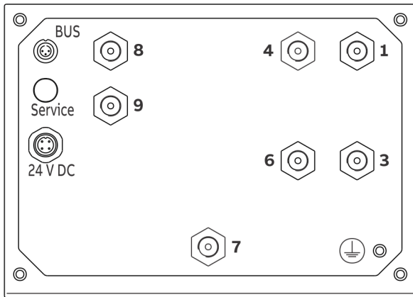
Figure 5: Gas connections Limas21 UV
