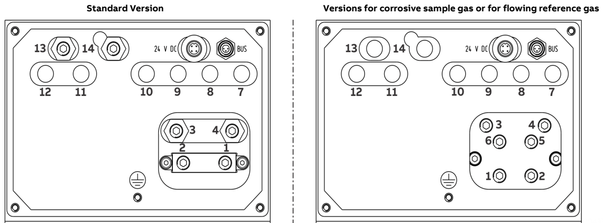
Figure 11: Gas connections Caldos25
