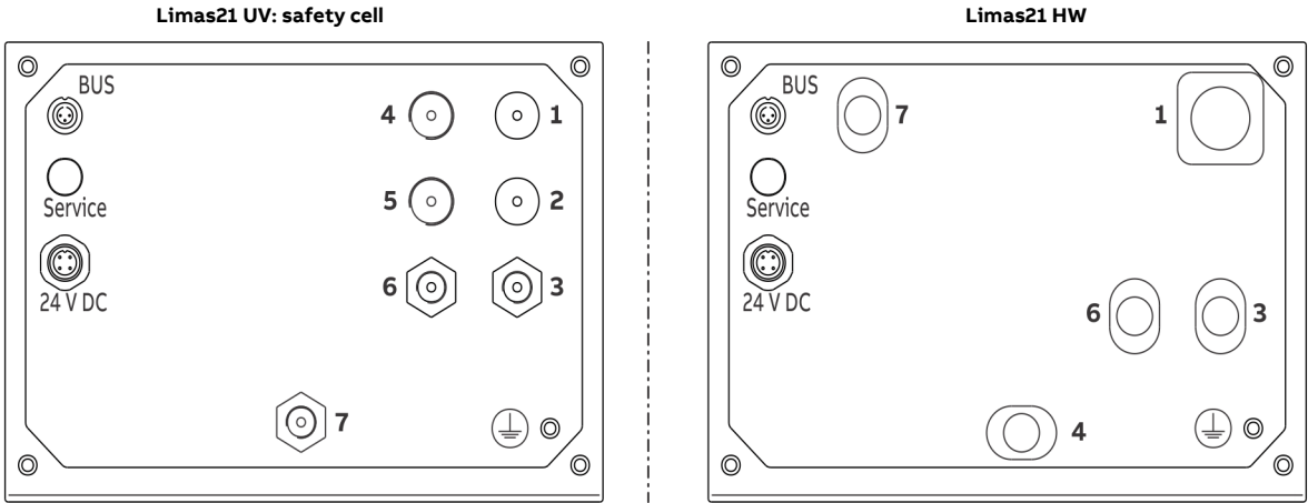
Figure 6: Gas connections Limas21 UV+HW
