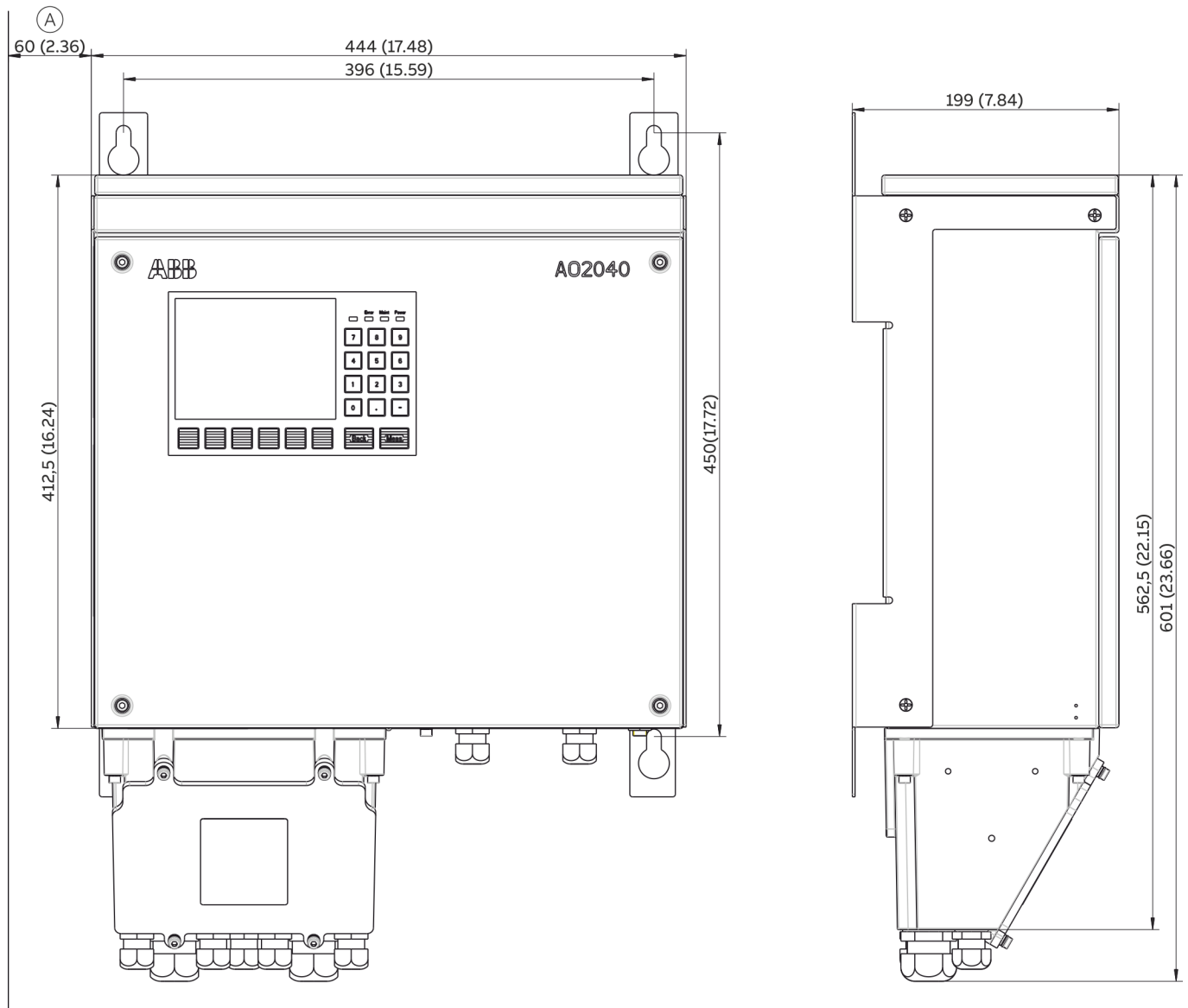
Figure 26: AO2040 dimensions
