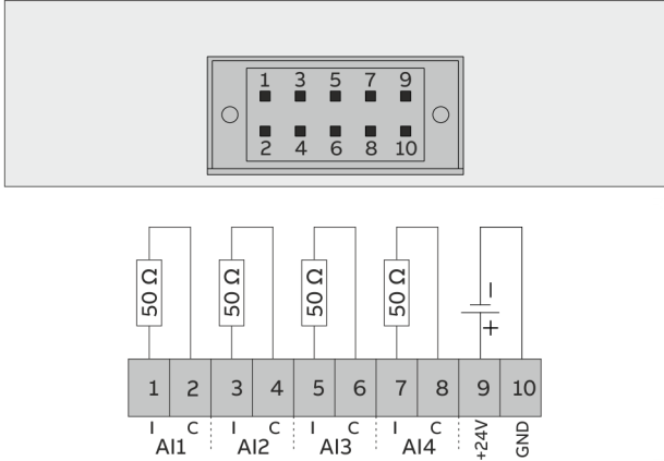
Figure 24: Analog input module
