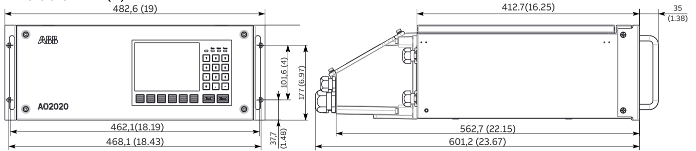
Figure 25: AO2020 dimensions
