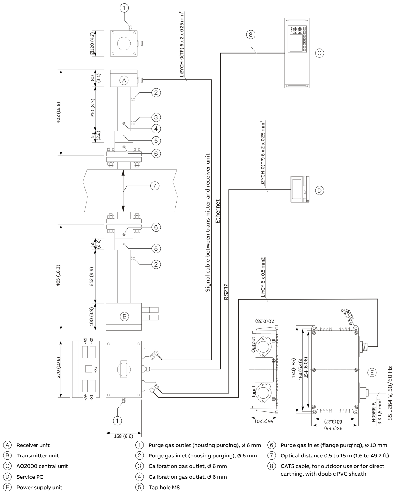
Figure 2: Block diagram of AO2000-LS25
