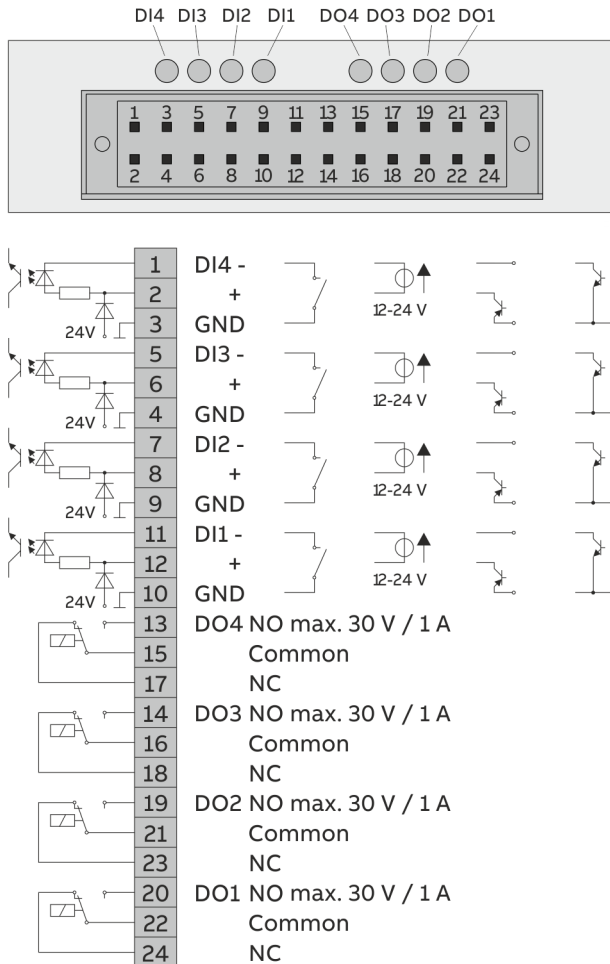
Image 21: Electrical connections, digital I/O module
