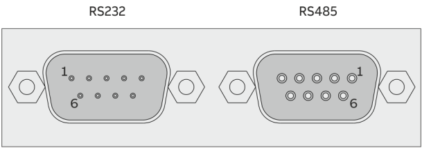
Figure 20: Modbus module
